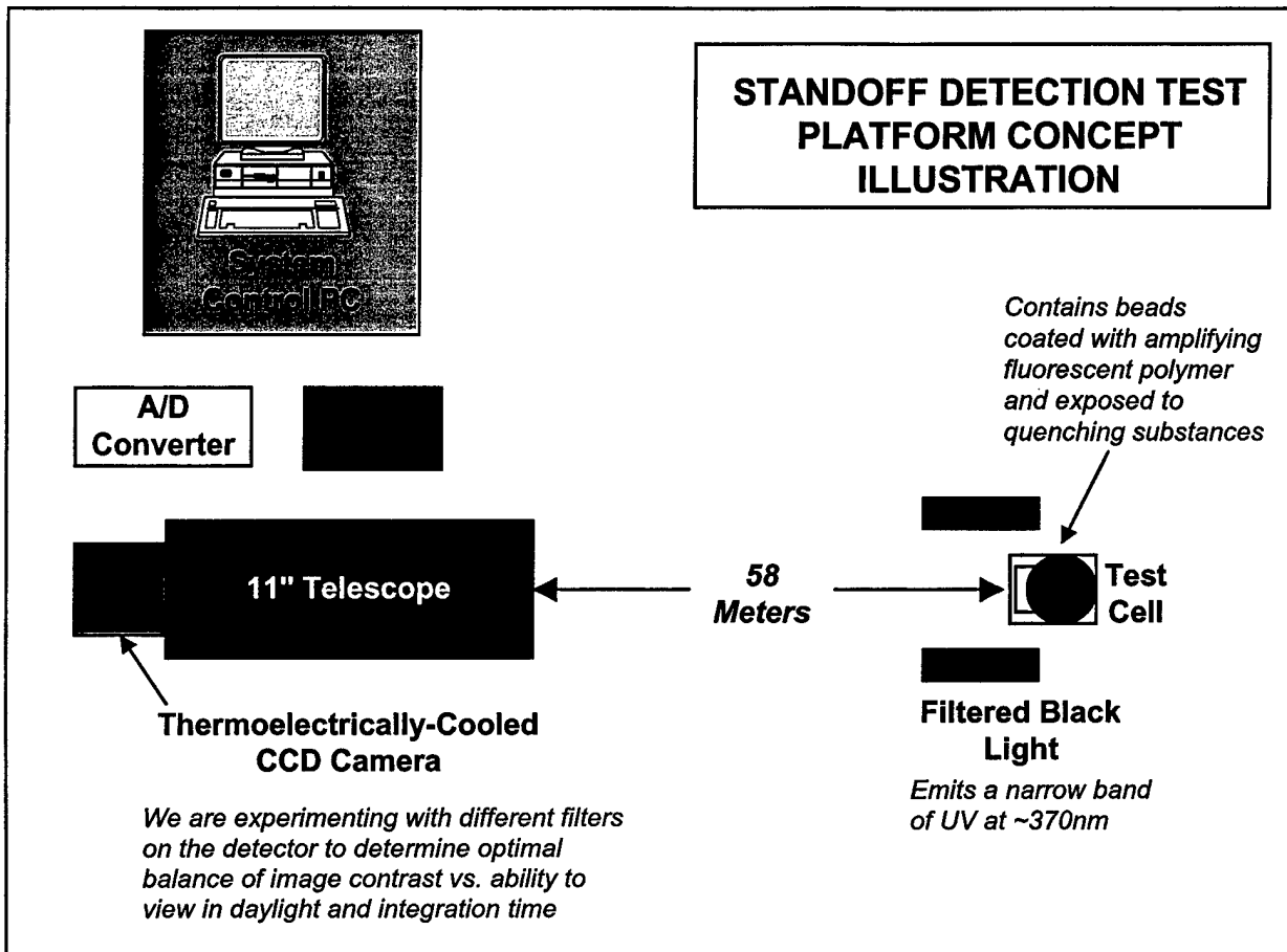
Figure 10. Optical test bed system diagram.
